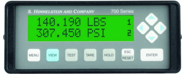
Model 766+ - 2 channel dc current signal conditioner - for torque, speed, flow, pressure, and temperature transmitters.
